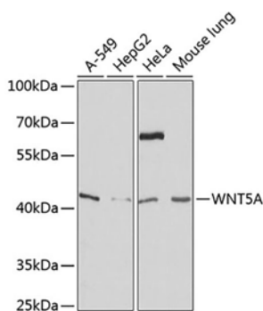
Fig. 1. Western blot analysis of extracts of various cell lines, using WNT5A antibody at 1:3000 dilution. Secondary antibody: HRP-labeled Goat Anti-Rabbit IgG(H+L) (A0208) at 1:1000 dilution. Lysates/proteins: 25µg per lane. Blocking buffer: QuickBlock™ Blocking Buffer (P0231). Detection: BeyoECL Star (P0018A). Exposure time:1s.
